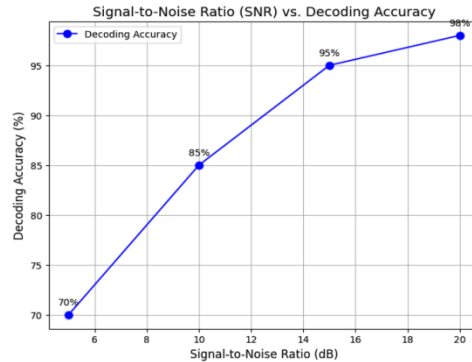
Figure 4: Graph: Signal-to-Noise Ratio (SNR) vs. Decoding Accuracy
