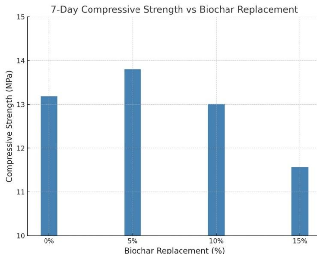
Figure 6: 7-Day Compressive Strength
