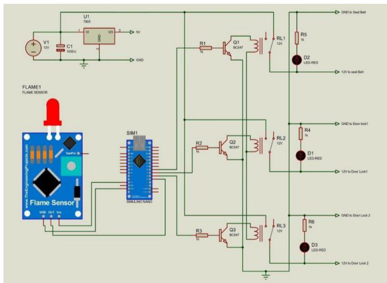
Figure 4: Circuit Diagram
