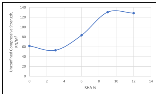
Figure 16: Effect of RHA on UCS of Soil
