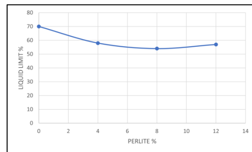
Figure 7: LL of Soil + RHA + Perlite Sample
