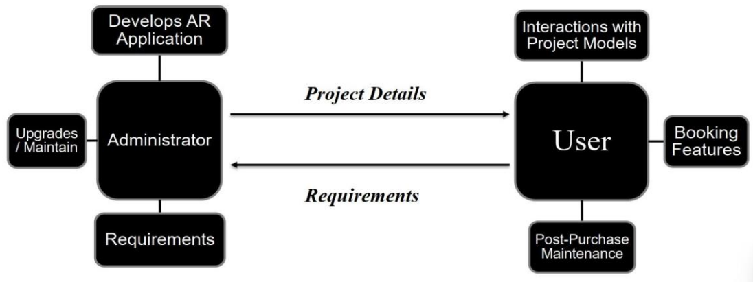
Figure 1: Architecture
