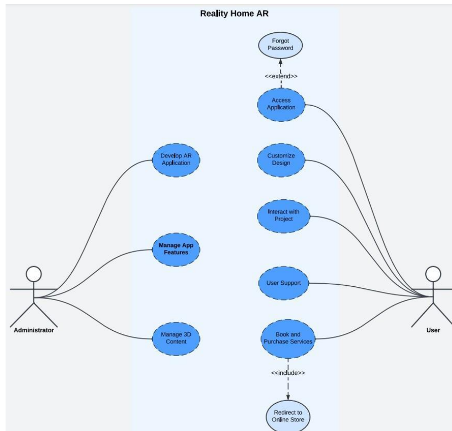
Figure 2: Usecase Diagram
