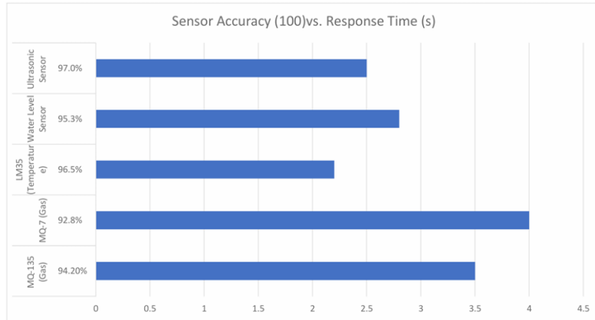
Figure 1.1: Sensor Accuracy and Response Time Analysis.
