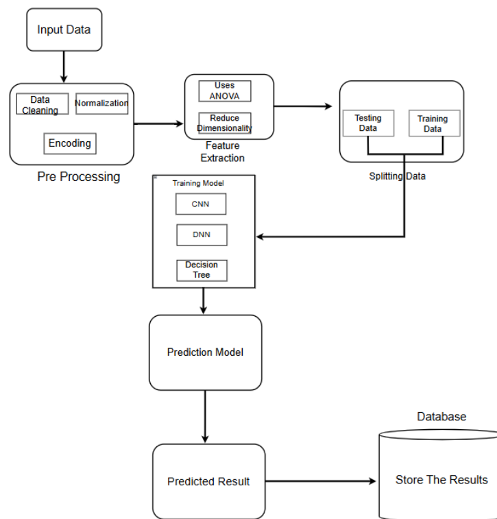
Figure 1: Methodology
