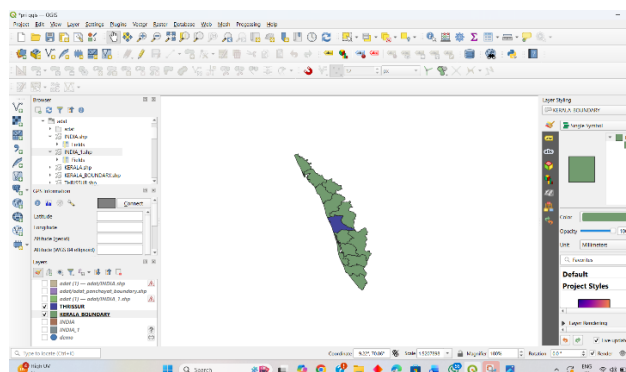
Figure 4: Location of study area in Kerala
