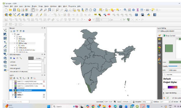
Figure 3: Location of study area in India
