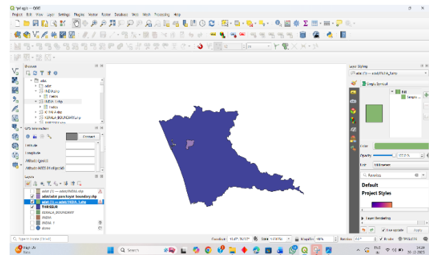
Figure 5: Location of study area Thrissur District
