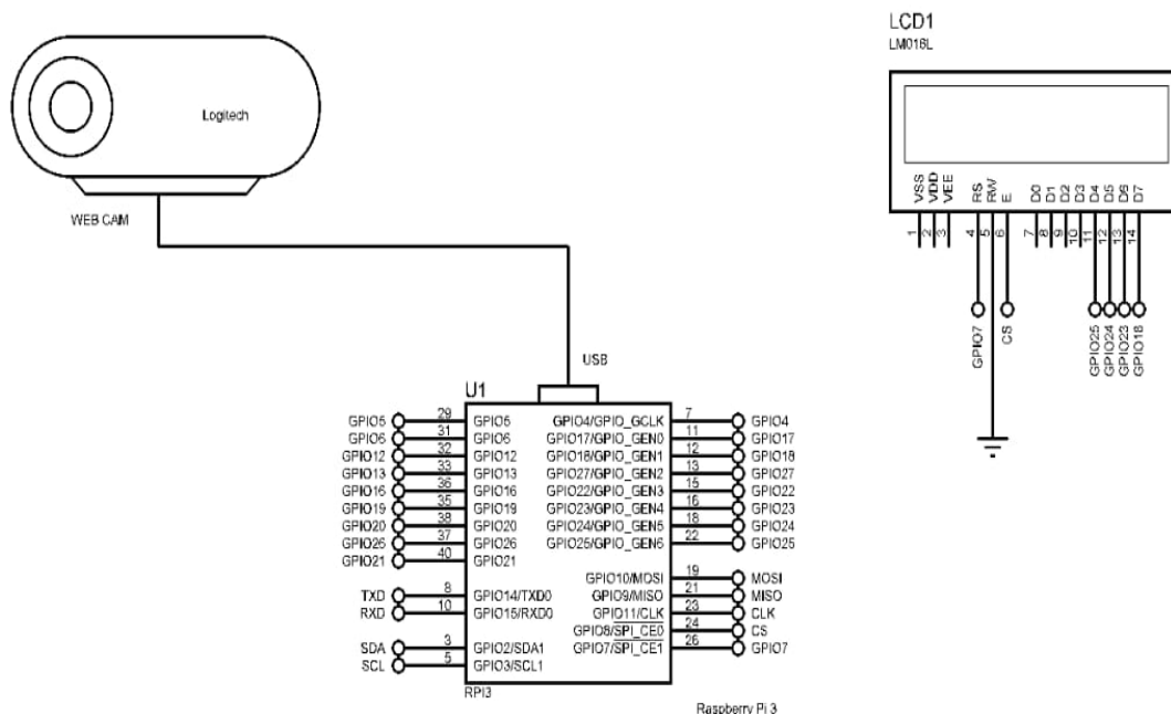
Figure 2: circuit diagram of AI powered face recognition and attendance system
