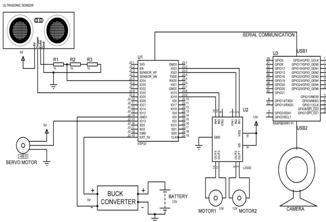
Figure 2: Circuit Diagram of the System
