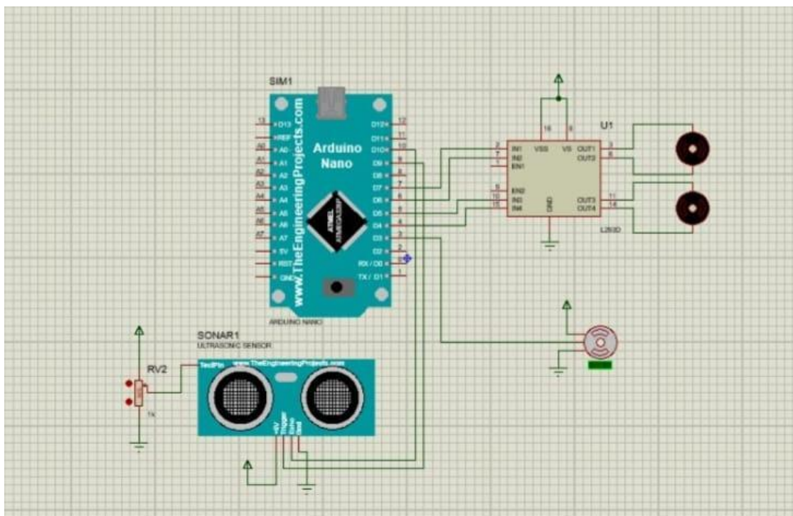
Figure 3: Simulation Using Proteus Software
