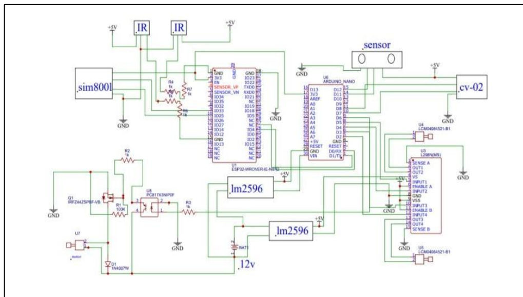
Figure 2: Circuit Diagram
