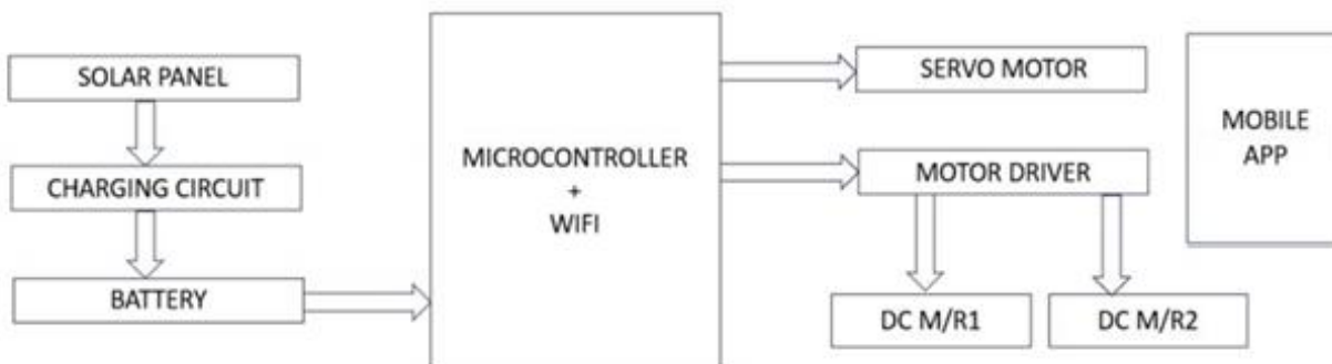
Figure 1: Flowchart Of Solar Powered Seed Sowing Machine
