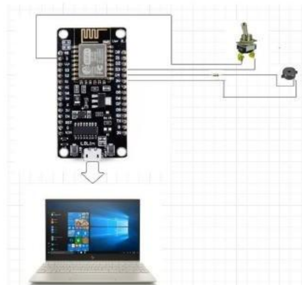
Figure 1: Experimental Setup of the proposed Advanced Blind Assistance System.
