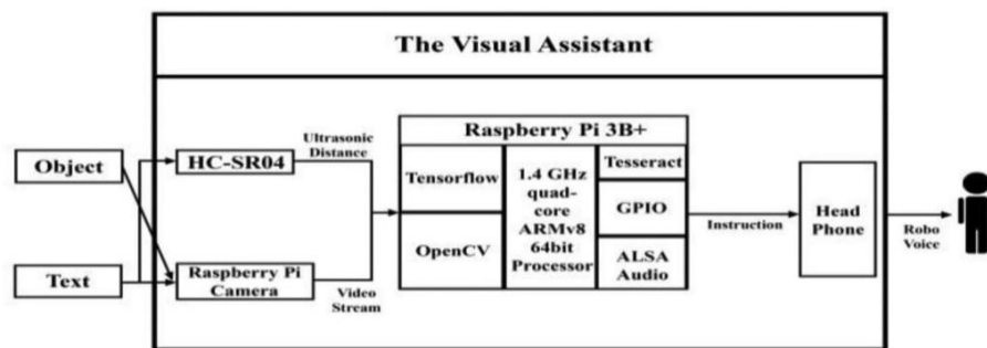
Figure 1: Block Diagram of Visual Assistant
