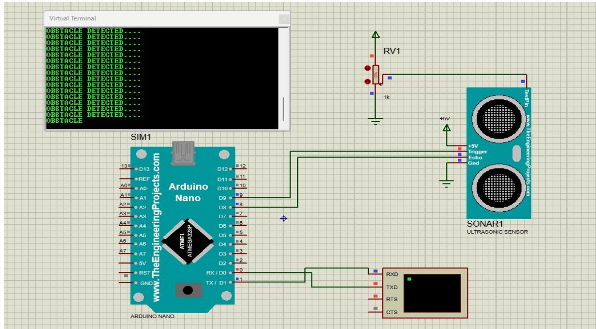
Figure 4: Simulation Using Proteus Software
