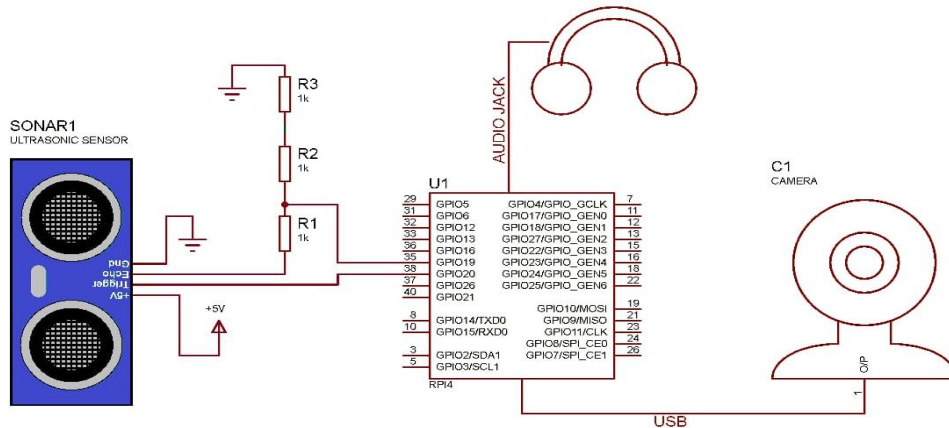
Figure 3: Circuit Diagram of the System
